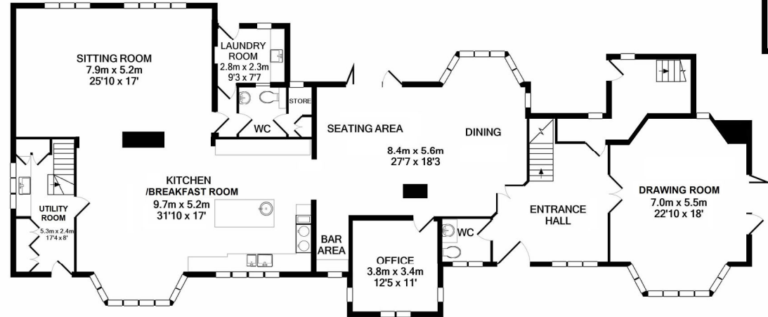
GROUND FLOOR
